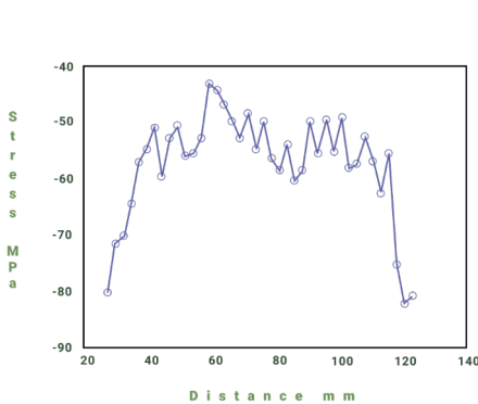
Stress Uniformity Graph
